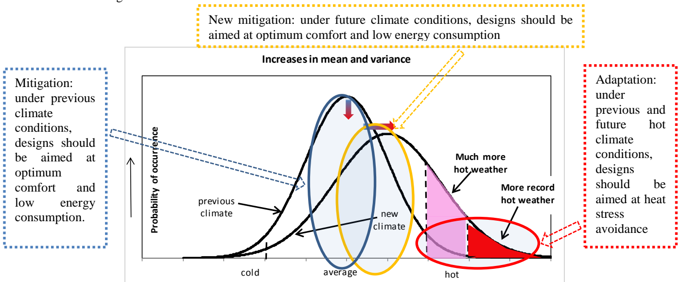
Figure 1: Schematic depiction of the effects on extreme temperatures when both the mean and variance increase for a normal temperature distribution based on an IPCC report [15]
